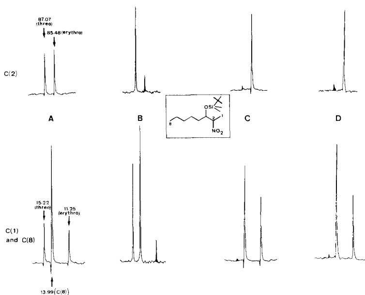
Fig. 1. 13 C-NMR. Spectra of 3-(1-butyl)dimethylsilyloxy-2-nitrooctane ( 15 ) obtained via different routes. A : from classical Henry reaction followed by O -silylation; B : from low-temperature protonation of the dilithio derivative 28 ( R^1 = C_5H_{11} , R^2 = CH_3 ) followed by O -silylation; C : from low-temperature protonation of the nitronate 35 ( R^1 = C_5H_{11} , R^2 = CH_3 ) of O -silylated nitroaldol; D : from fluoride-catalyzed O -silylnitroaldol addition. The signals from the minor isomers are darkened for easy identification.
